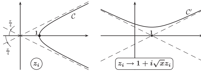
Figure 4. Contour of integration, \mathcal{C} , in equation (45) and its transformation into the contour \mathcal{C}' , right-hand side picture, according to the rule z_i \rightarrow 1 + i\sqrt{x}z_i .
