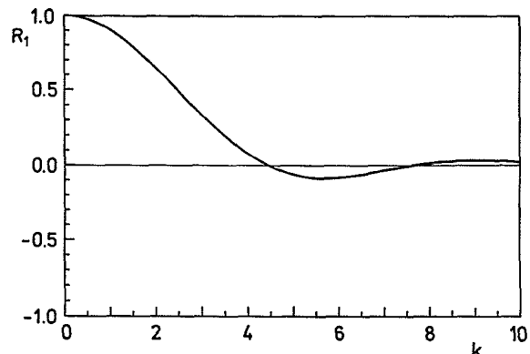
FIG. 5. Coefficient R_1 for the operator J_z calculated for different realizations of the kicked top in the transition region between regularity ( k \leq 4 ) and chaos ( k \geq 4 ); j=50, \beta=1.7 .
