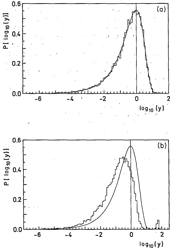
FIG. 1. Distribution of squares of absolute values of matrix elements for the operators (a) J_z and (b) J_z^2 in the Floquet basis of the kicked top. Solid lines correspond to the \chi_1^2 distribution provided by random-matrix theory. Total angular-momentum number j=100 and coupling constants k=10.0 , \beta=1.7 .
