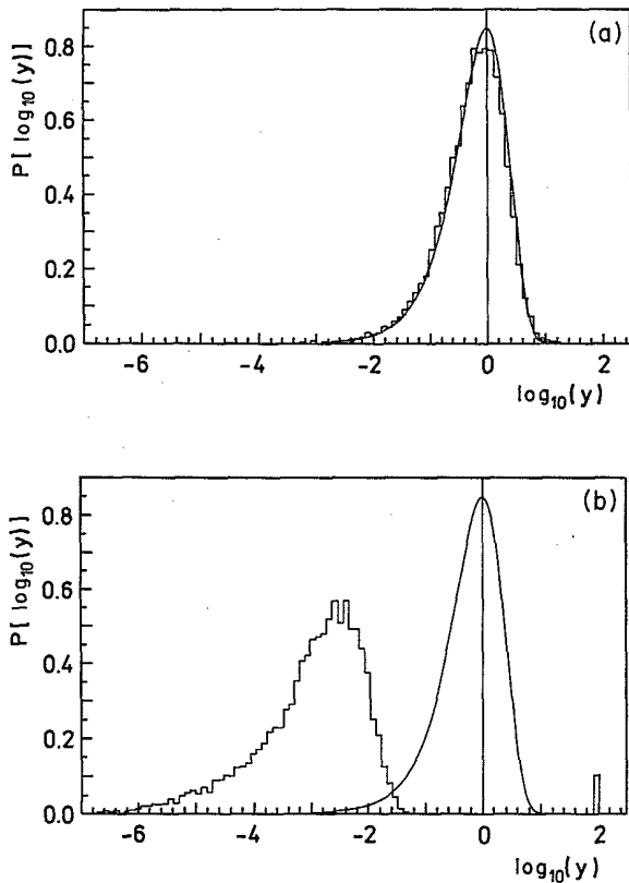
FIG. 3. Distribution of squares of absolute values of matrix elements for the operator V=\exp(-idJ_z) in the Floquet basis of the kicked top for (a) d=0.04 and (b) d=0.001 ; system parameters as in Fig. 1. Solid lines correspond to the predictions of random-matrix theory.
