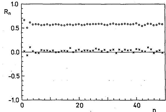
FIG. 2. Coefficients R_n for the operators J_z (asterisks) and J_z^2 (circles). Total angular-momentum number j=50 , other parameters as in Fig. 1.
