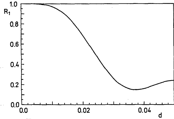
FIG. 4. Coefficient R_1 for the operator V=\exp(-idJ_z) as a function of the parameter d .
