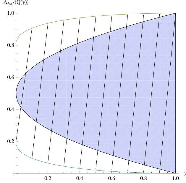
Fig. 3. The shaded region is the product higher rank numerical range of Q(\gamma) given by Eq. (95). The hatched region in which it is included is the bound stemming from the application of Theorems 17 and 18.
