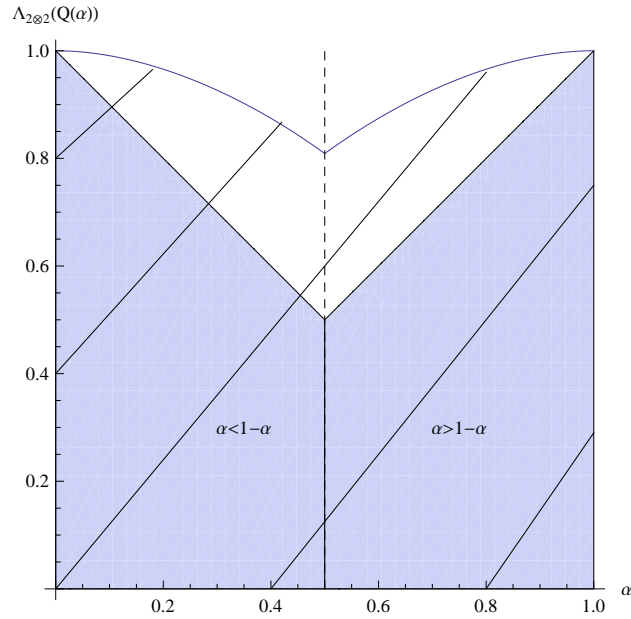
Fig. 2. The shaded region is the 2 \otimes 2 range of Q(\alpha) given by Eqs (75-78). The hatched region is the bound from Theorems 17 and 18.
