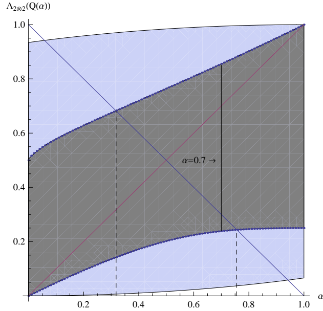
Fig. 1. The light shaded region represents the bound given by Eq. (66) in the whole range of \alpha , the dark grey region is the bound given by Eq. (69) (the dots are for \lambda_{\uparrow, \downarrow}(\alpha) ). We have also put the section bounding the product range for an exemplary value \alpha = 0.7 . Additionally, we plotted the lines \alpha and 1 - \alpha . While the former value always belongs to the product range (as we have discussed in the main text) there is a range of \alpha , where the latter lies outside it with certainty as it is cut off by the bound, this cut off is represented by the dashed lines.
