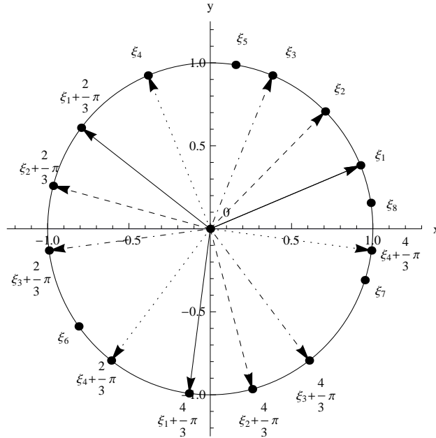
Fig. 5. Distribution of eigenvalues from Eq. (103) (for clarity we have written only phases). The arrows represent the summations of Eq. (106).
