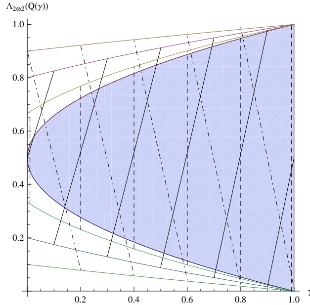
Fig. 4. The inner shaded region corresponds to \alpha = 1/2 in Property 15 and represents the true 2 \otimes 2 rank of Q(\gamma) given by Eq. (95). The region with dashed lines corresponds to \alpha = 1/3 , solid lines — \alpha = 1/5 , dot dashed lines — \alpha = 1/10 . In the limit \alpha \rightarrow 0 we will obviously get [0, 1] .
